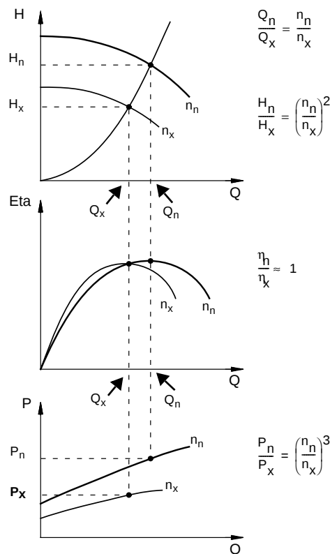
Fig. 20 Affinity equations
